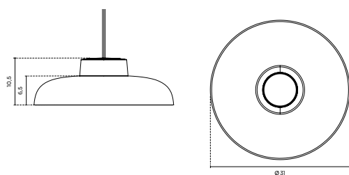
Measurements Split Straight Acorn
