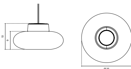
Measurements Split Round Orbit
