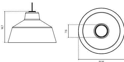
Measurements Ratio 39 Pendant Lamp
